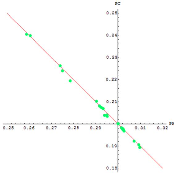
Fig. 1 In red, the line P_A + P_C = \frac{1}{2} , and in green, the observed points (P_A, P_C) for each human chromosome (colour figure online).
