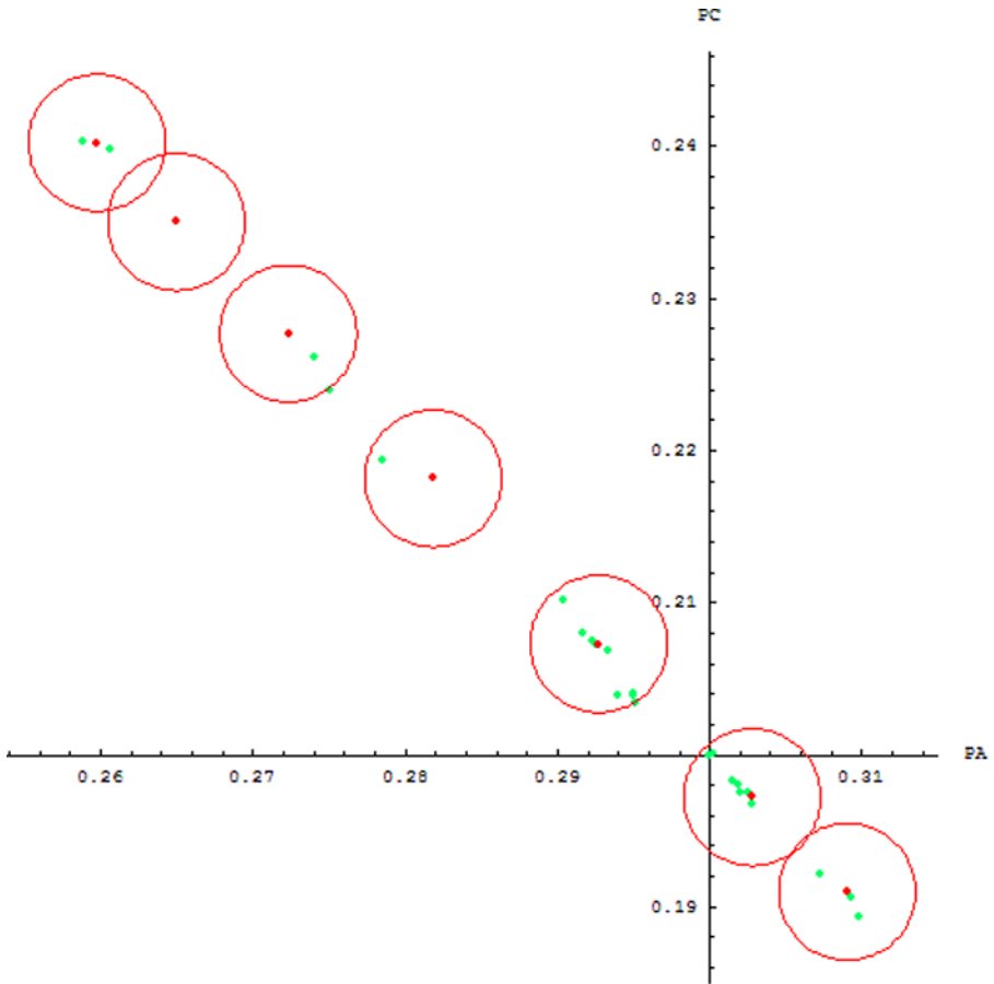
Fig. 2 In red dots, the solutions of the optimization problem for different values of k . In green, the points (P_A, P_C) for each one of the human chromosomes (colour figure online).
